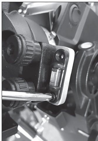
Figure 2. Remove the two black Philips screws to remove the bubble level.
