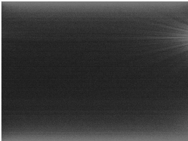
Figure 10. A 120 second dark frame. From a G10. Note the amp glow on the upper right side, this is standard for the ICX294 chip, and is removed from light images during dark frame subtraction. The G16 will show a different dark frame amp glow signature.
