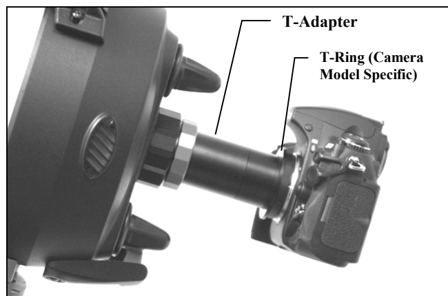
Figure 3-1 – T-Adapter for 8" Optical Tube
