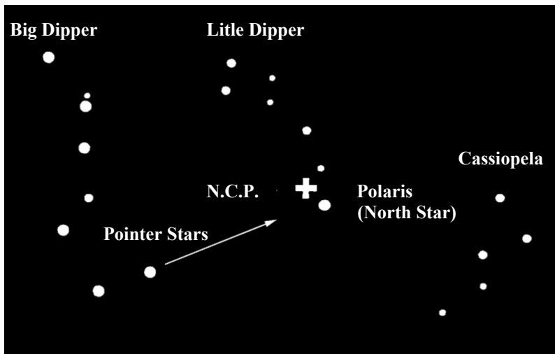
Figure 4-6 The two stars in the front of the bowl of the Big Dipper point to Polaris which is less than one degree from the true (north) celestial pole. Cassiopeia, the “W” shaped constellation, is on the opposite side of the pole from the Big Dipper. The North Celestial Pole (N.C.P.) is marked by the “+” sign.
