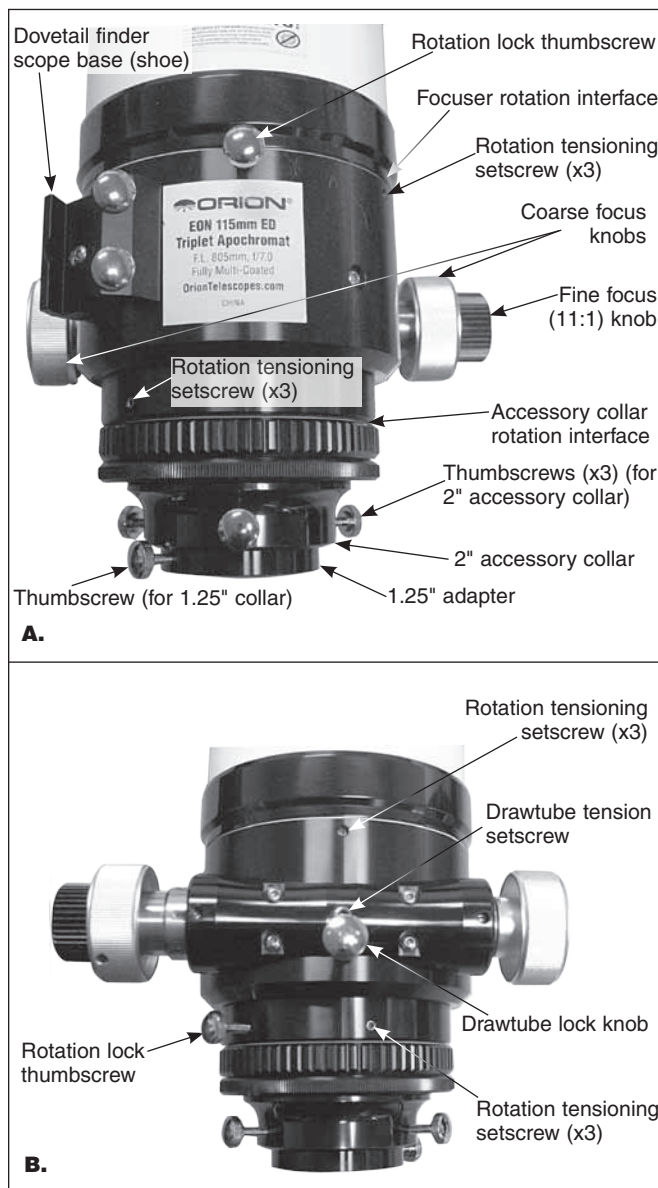
Figure 2. The 3" dual-speed Crayford focuser used on both the EON 115 and 130 A) Top side, B) bottom side
