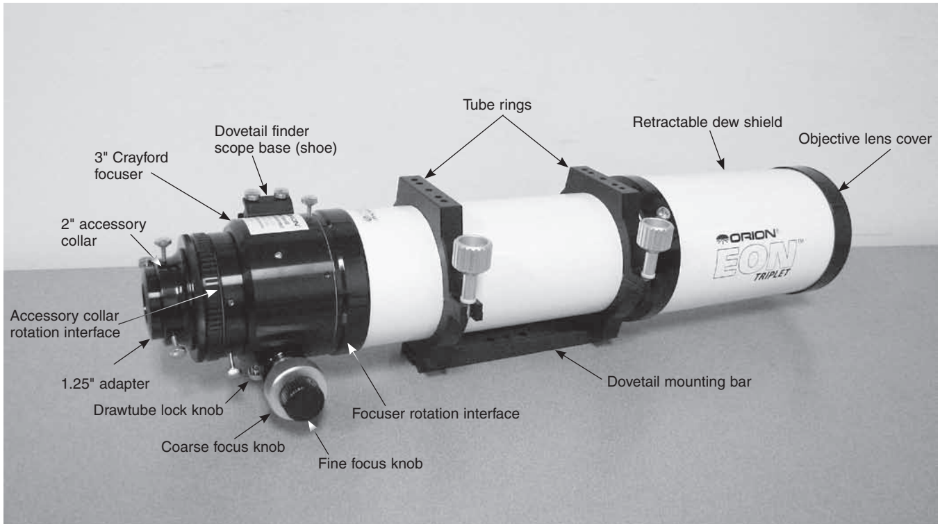
Figure 1. Features and components of the EON Triplet apochromatic refractor
