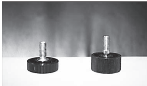
Figure 1: The vertical stop knob on the left has a thinner head. This is the correct vertical stop knob to use. The knob on the right is incorrect and should be discarded.
