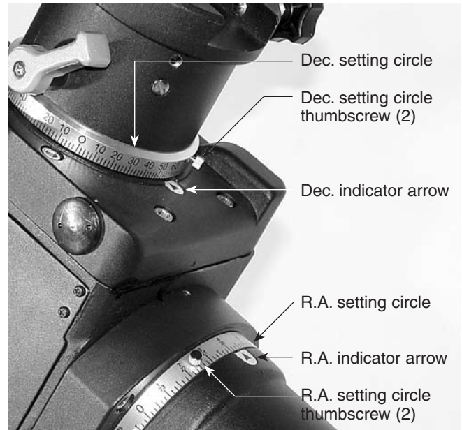
Figure 12. The R.A. and Dec. setting circles.
