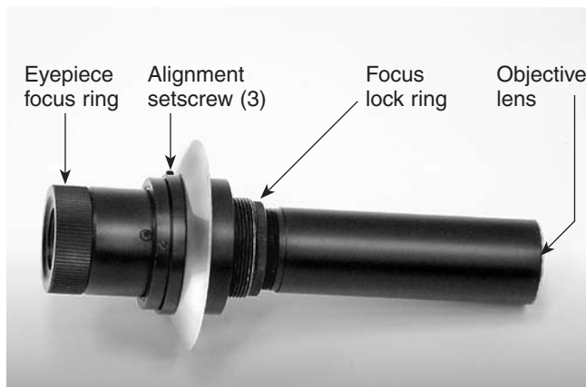
Figure 9. The optional polar axis finder scope.
