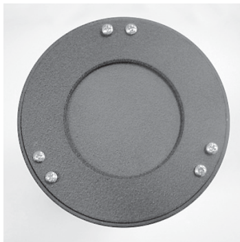
Figure 11. The back end of the optical tube (bottom of the primary mirror cell). The three pairs of collimation screws adjust the tilt of the primary mirror.
