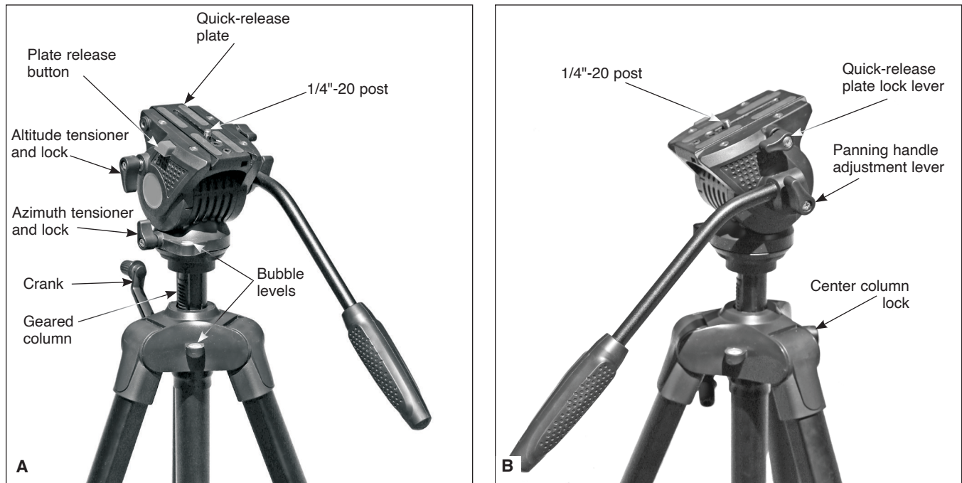
Figure 2. (A) The Tritech II pan head, left side and (B) right side.
